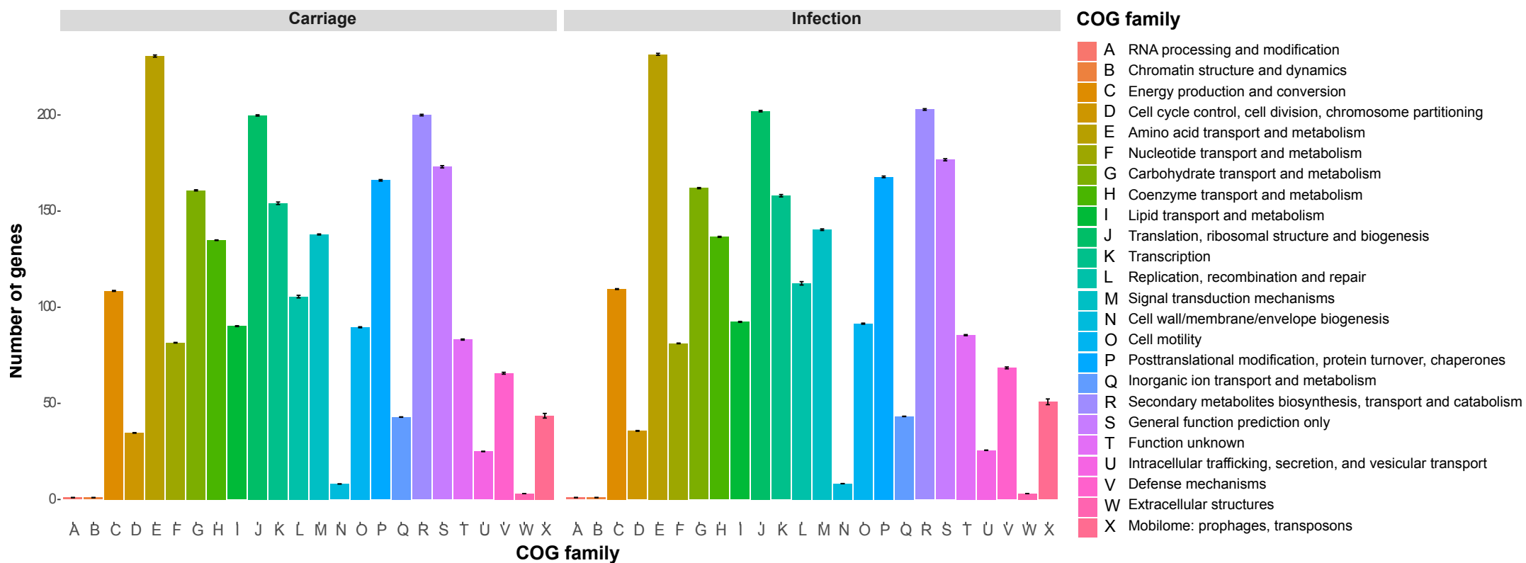
Supplemental Figure S9: Functional distribution of CDS according to COG between strains isolated from human carriage or during infection . The charts represent mean number assigned to each categories. The right strip indicates the different categories assigned with COG.
