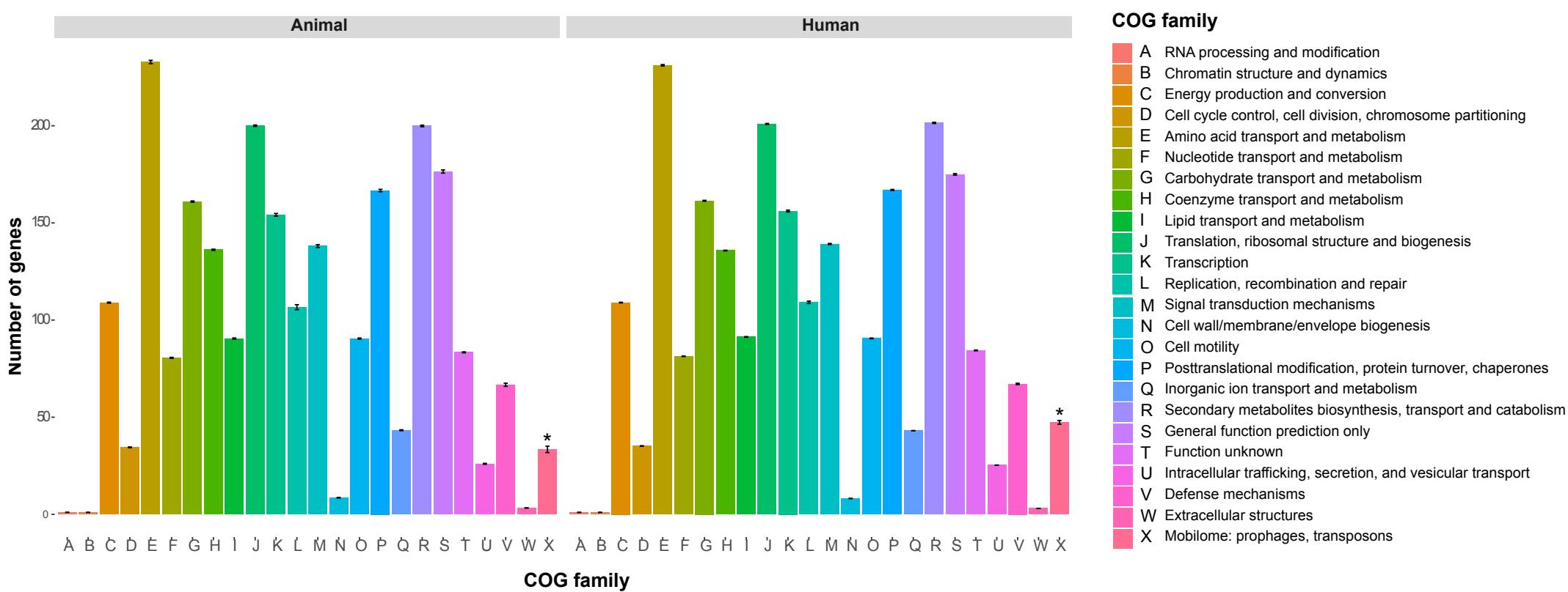
Supplemental Figure S7: Functional distribution of CDS according to COG between strains isolated from animal and humans. The charts represent mean number assigned to each categories. The right strip indicates the different categories assigned with COG.
